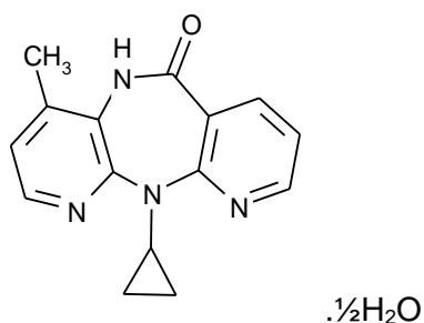
Nevirapine hemihydrate
