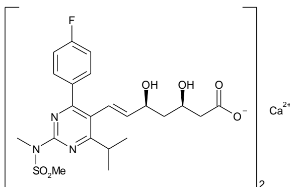
Figure 4 Chemical structure/general structure of rosuvastatin calcium
